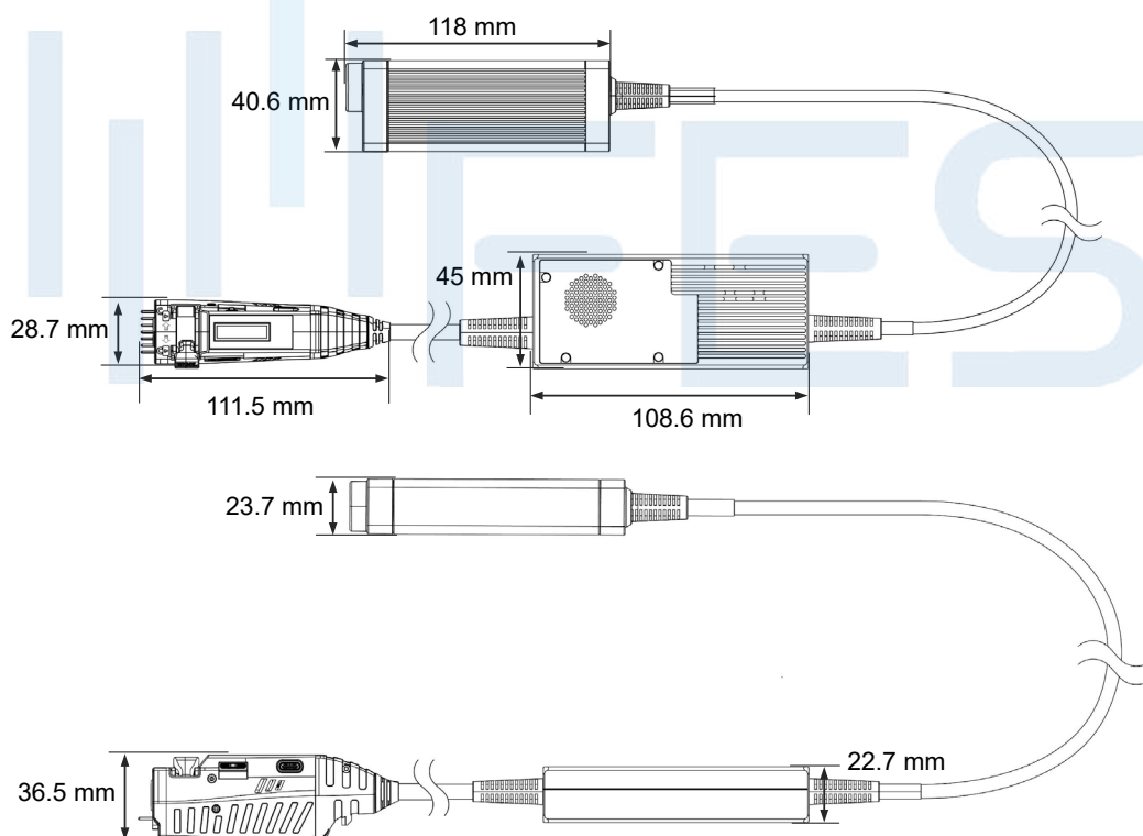
Figure 4.2 Probe Size
