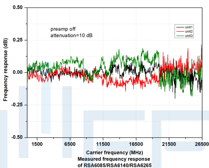
Frequency Response (attenuation = 10 dB, PA off)
