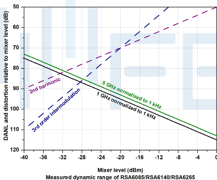
Distortion
