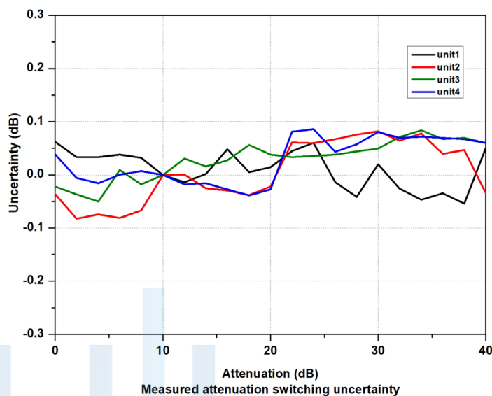
Switching Uncertainty
