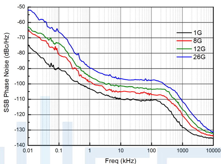
SSB Phase Noise
