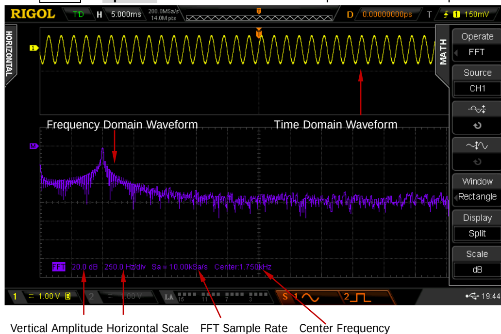
Figure 6-1 FFT Operation
