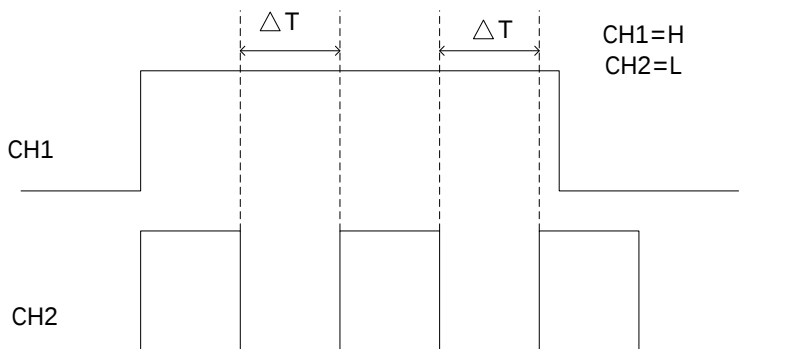
Figure 5-11 Duration Trigger
