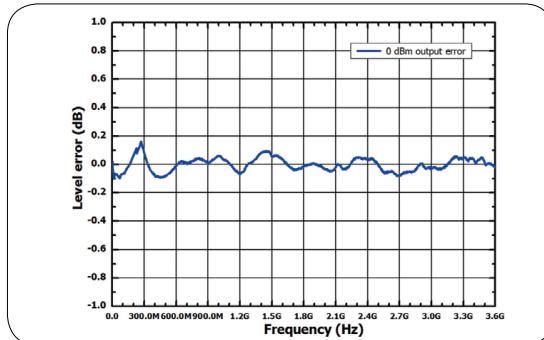
Measured at 0 dBm, level error vs. frequency
