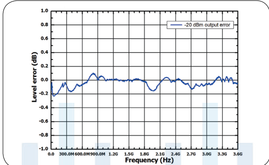
Measured at -20 dBm, level error vs. frequency
