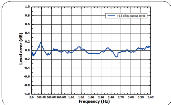
Measured at +13 dBm, level error vs. frequency
