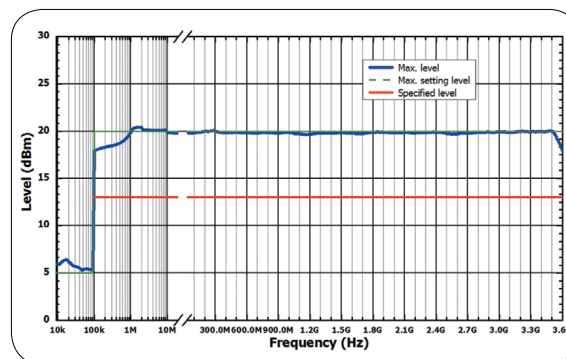
Measured maximum level vs. frequency
