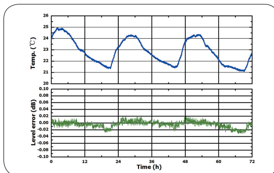
Measured level repeatability @ 1 GHz, 0 dBm
