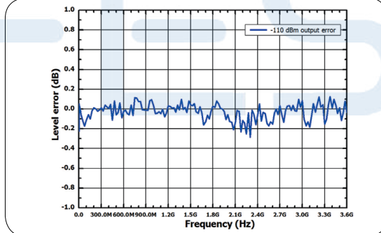
Measured at -110 dBm, level error vs. frequency
