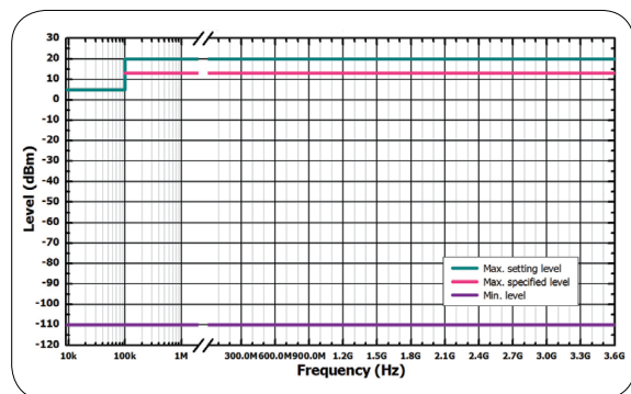
Maximum and minimum level vs. frequency
