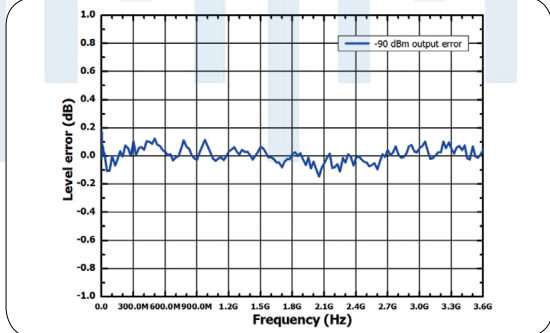
Measured at -90 dBm, level error vs. frequency
