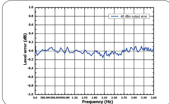
Measured at -60 dBm, level error vs. frequency
