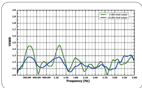
Measured VSWR vs. frequency
