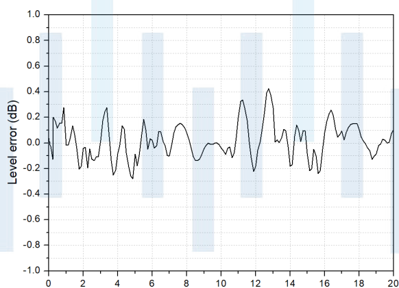
Measured at +10dBm, level error vs frequency
