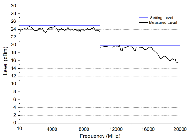
Measured maximum level
