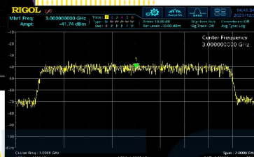
Multi-channel Synchronization
