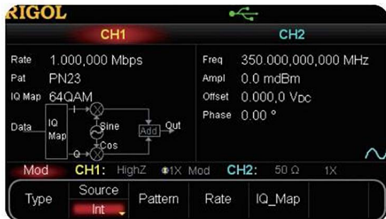
IQ Modulation
